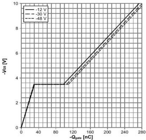
Figure 5: Gate-Charge Characteristics
